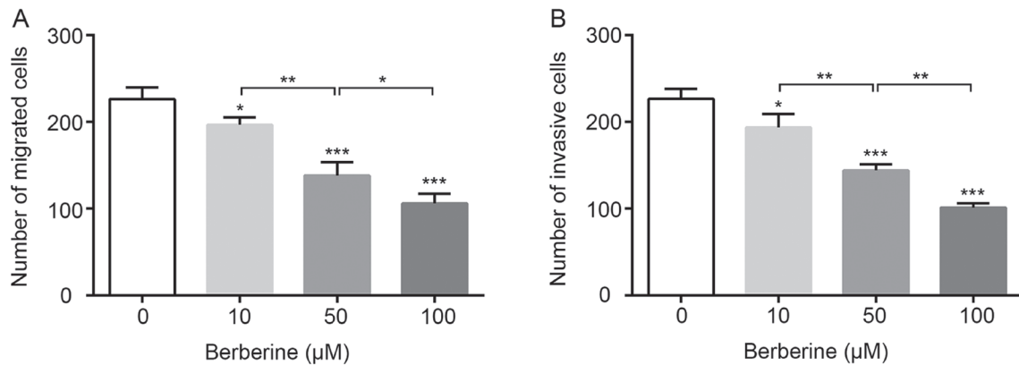
Fig. 2. The suppressive effect of berberine on cell migration and invasion in human Rb cells
